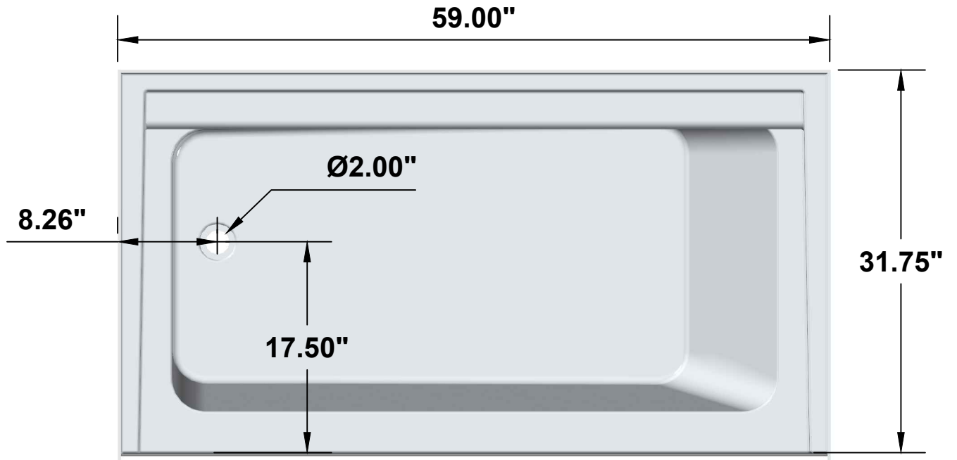
Top View
