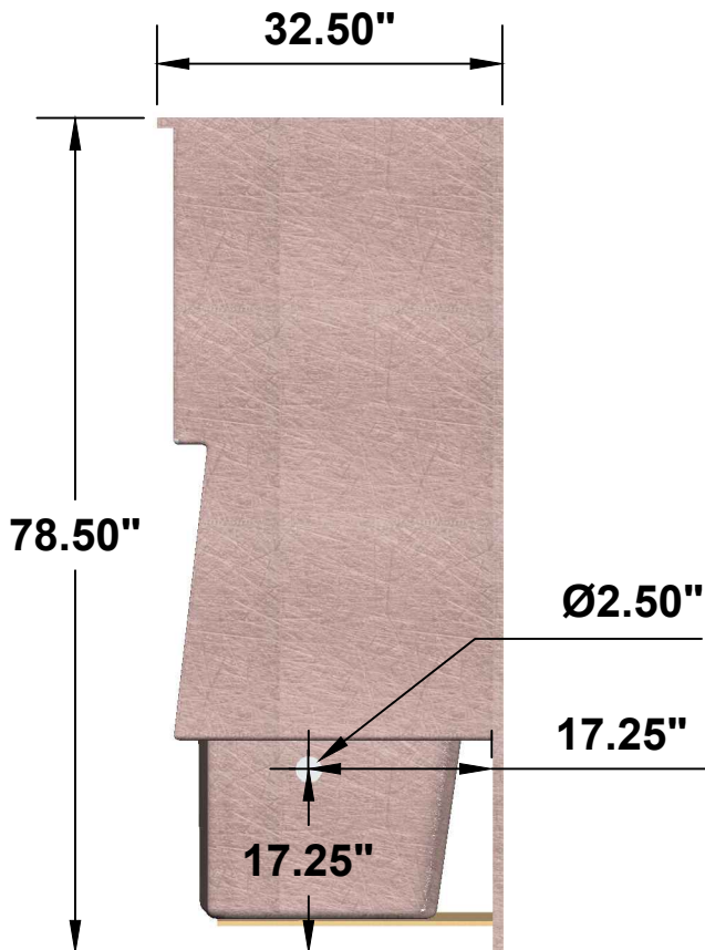
Side View
